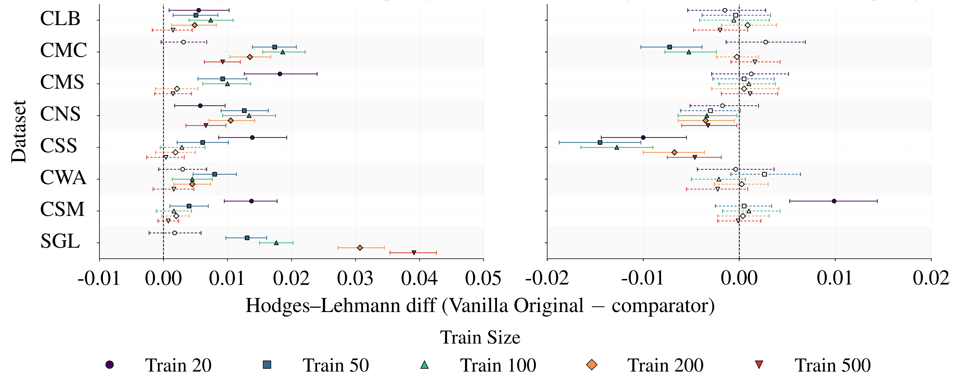
Vanilla Original vs Vanilla Topological
