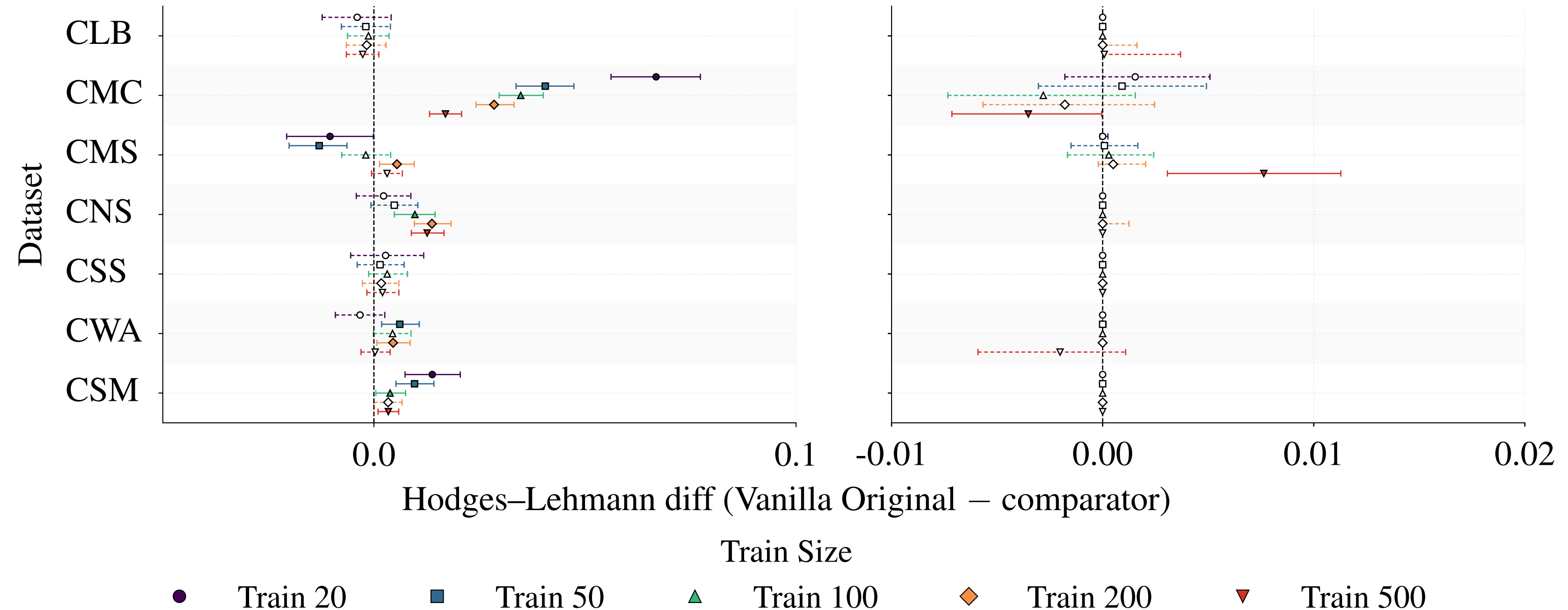
Vanilla Original vs oracle-PDAG
