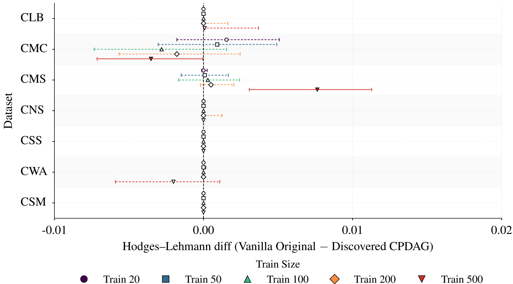
Vanilla Original vs Discovered CPDAG · NNAA (test – train)
