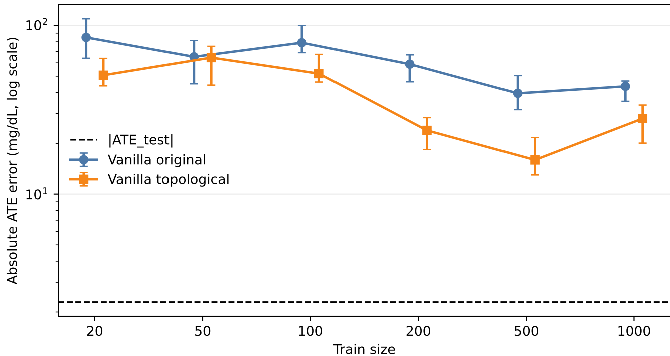
SimGlucose ATE Error on Outcome Scale
