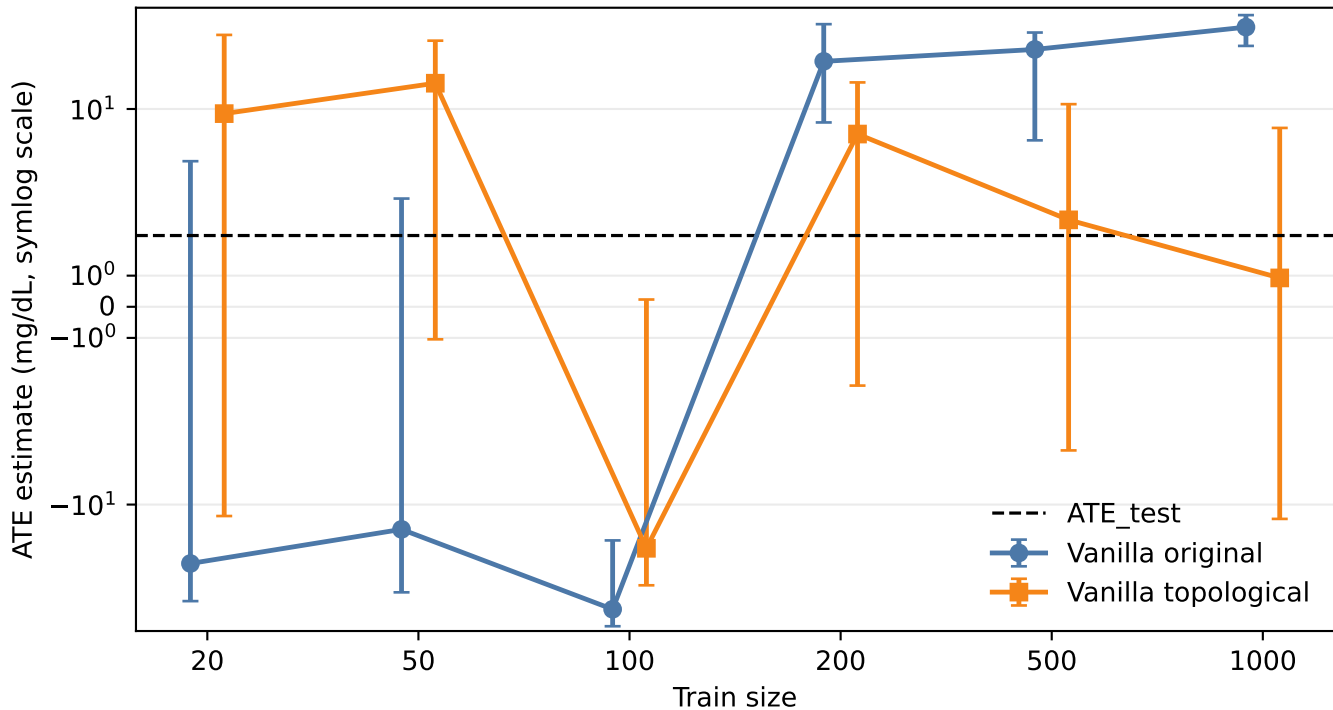
SimGlucose Synthetic ATE Estimates
