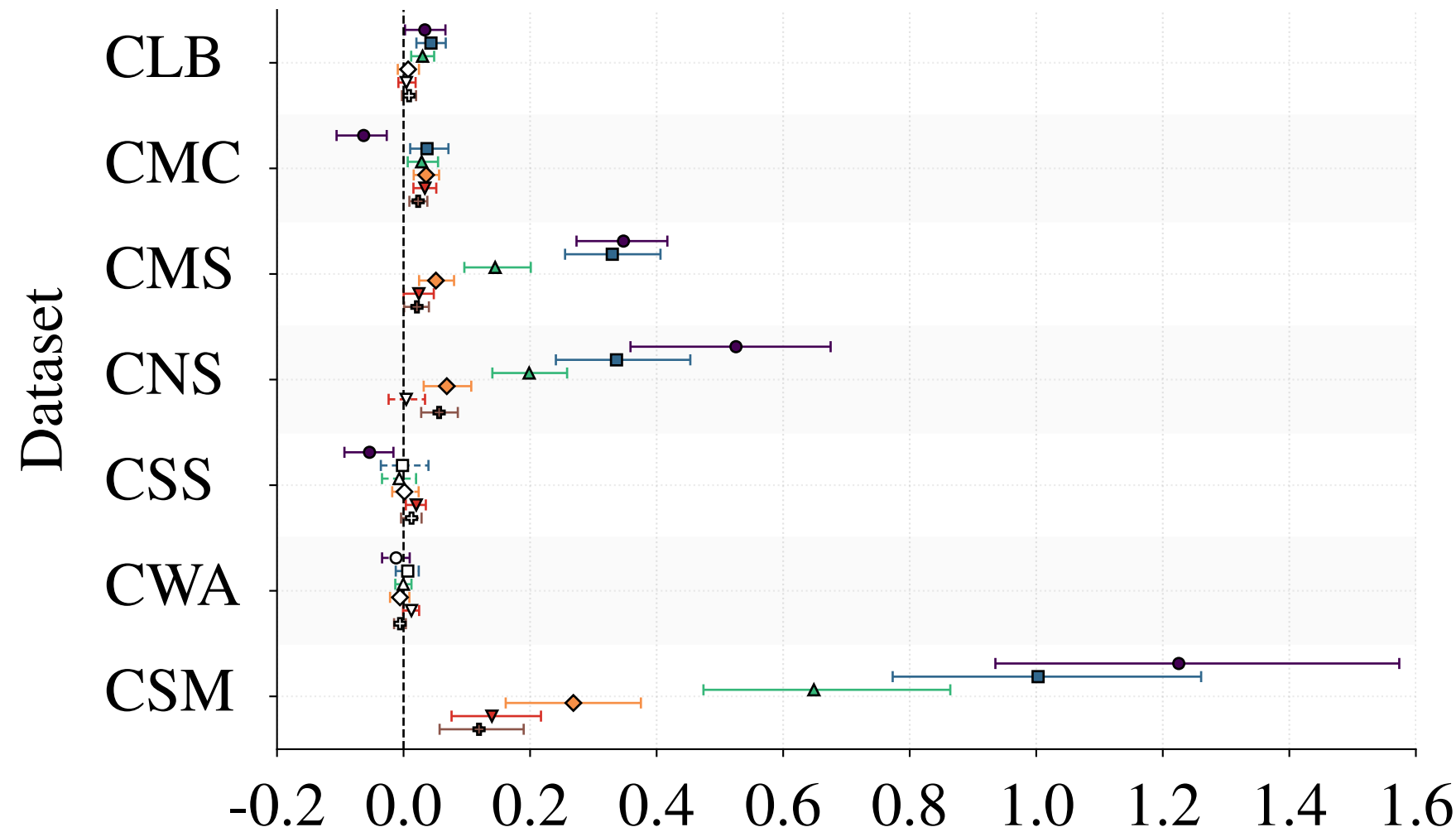
Vanilla Original vs DAG
