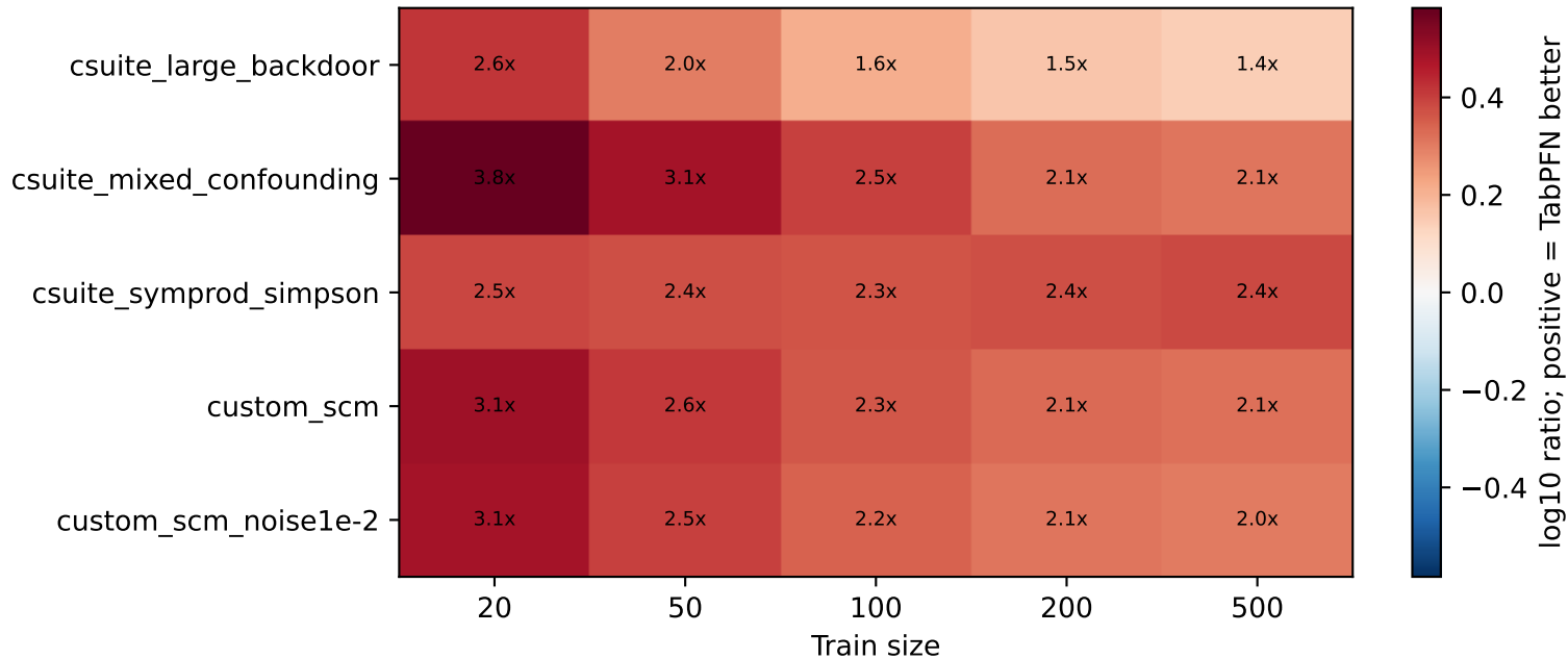
TabularARGN / TabPFN vanilla original median loss ratio - kMTVD
