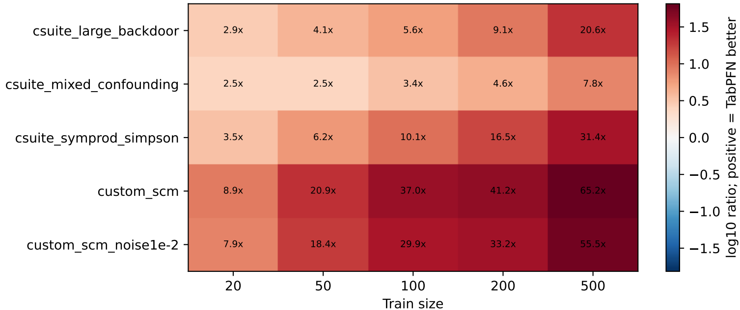
TabularARGN / TabPFN vanilla original median loss ratio - NNAE |x-0.5|
