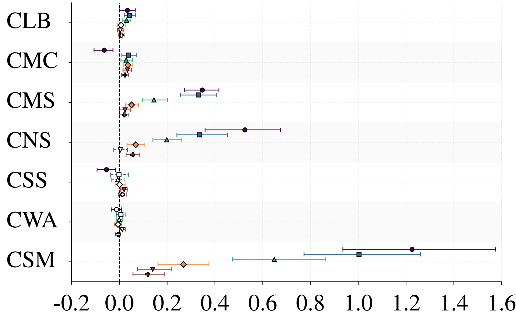
Absolute ATE Error |\text{Ground Truth} - \text{Estimate}| Vanilla Original vs DAG
