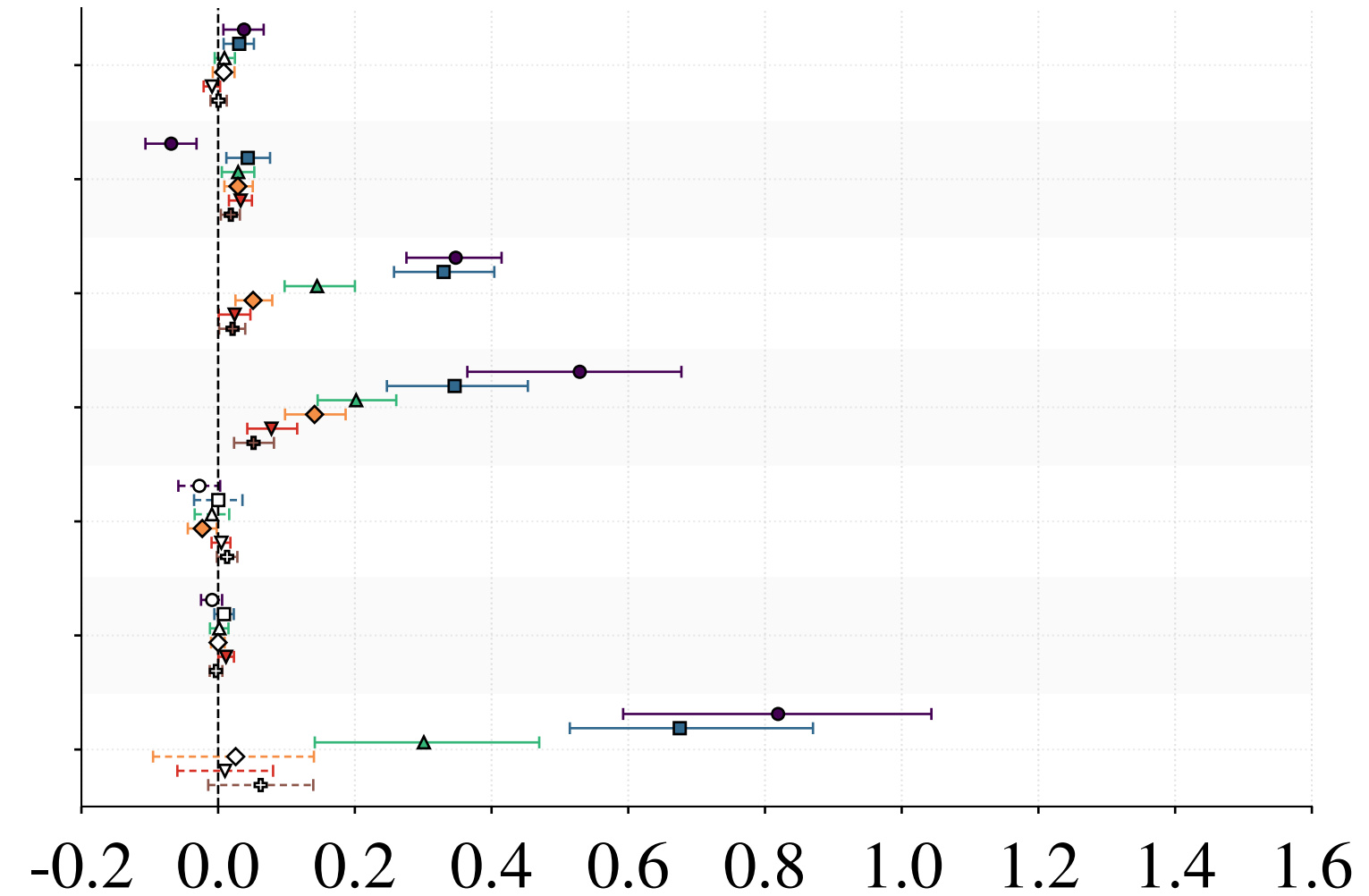
Absolute ATE Error |\text{Ground Truth} - \text{Estimate}| Vanilla Original vs DAG
