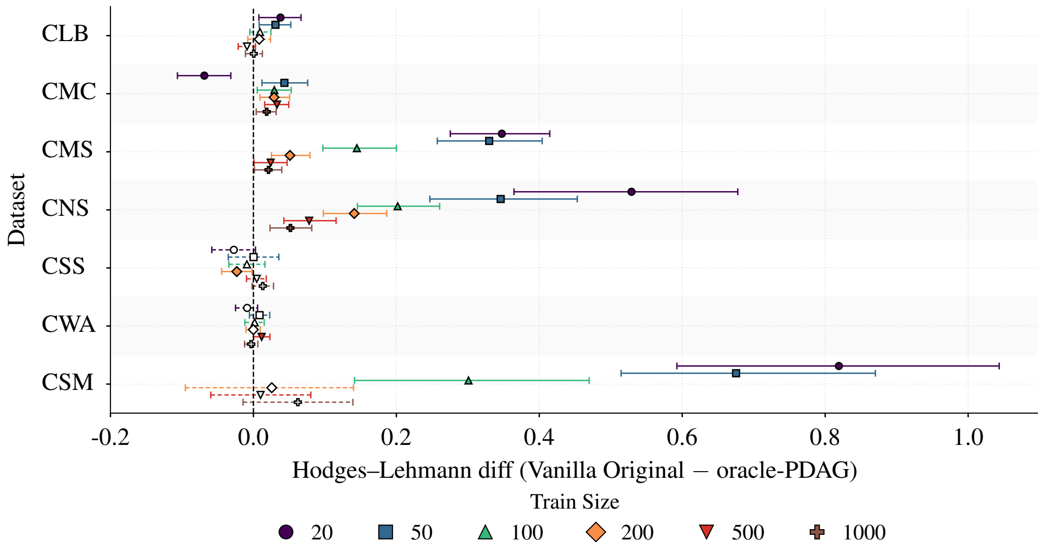
Vanilla Original vs oracle-PDAG Absolute ATE Error |\text{Ground Truth} - \text{Estimate}|
