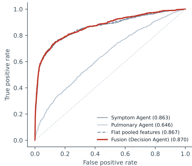
(a) ROC, out-of-fold
