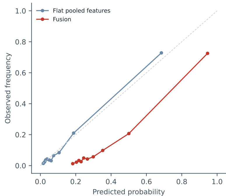
(c) Calibration
