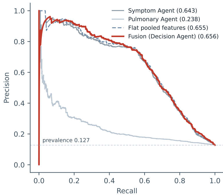
(b) Precision-recall
