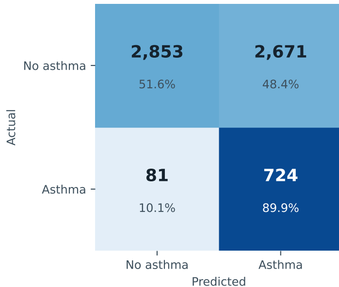
(b) Screening threshold (0.25)
