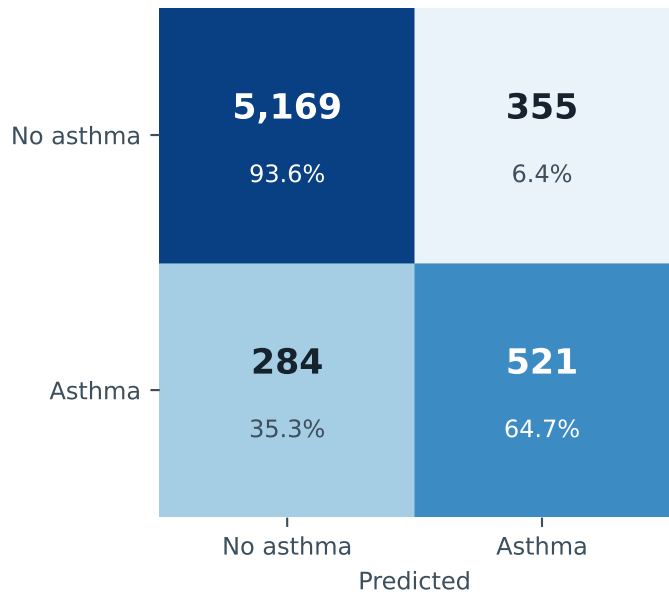
(a) Default threshold (0.50)
