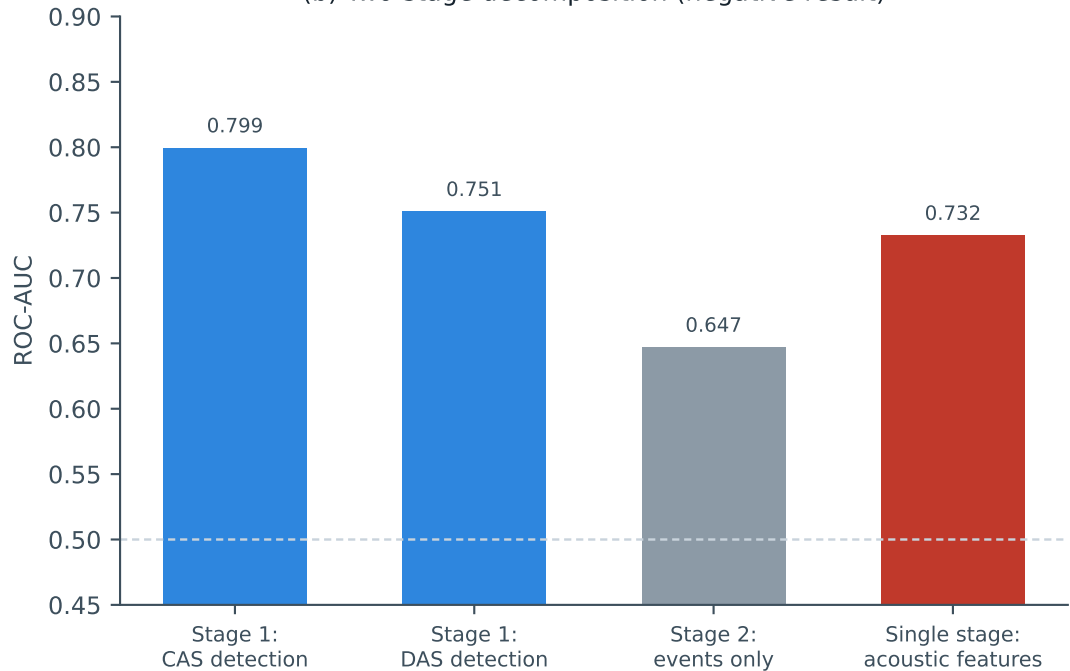
(b) Two-stage decomposition (negative result)
