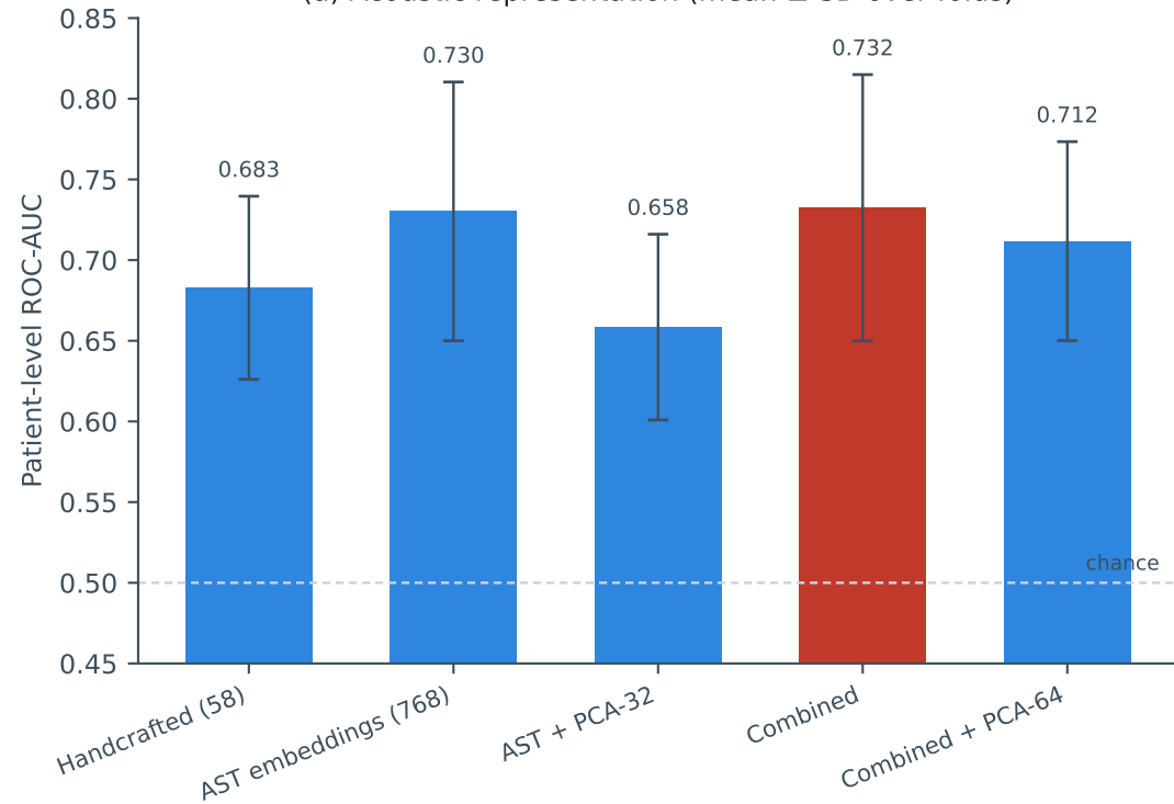
(a) Acoustic representation (mean \pm SD over folds)
