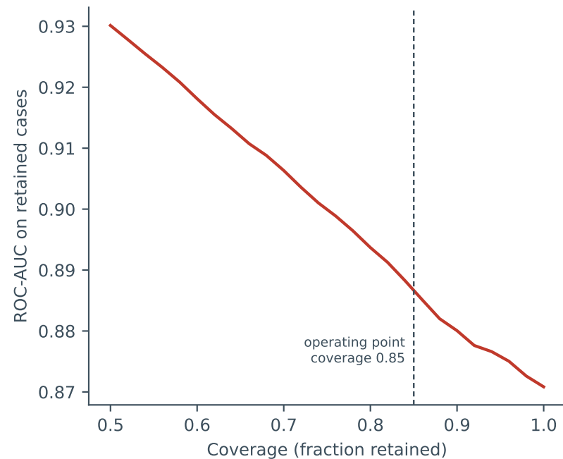
(a) Risk-coverage
