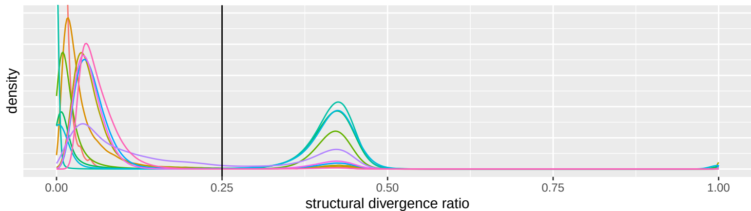
All datasets
