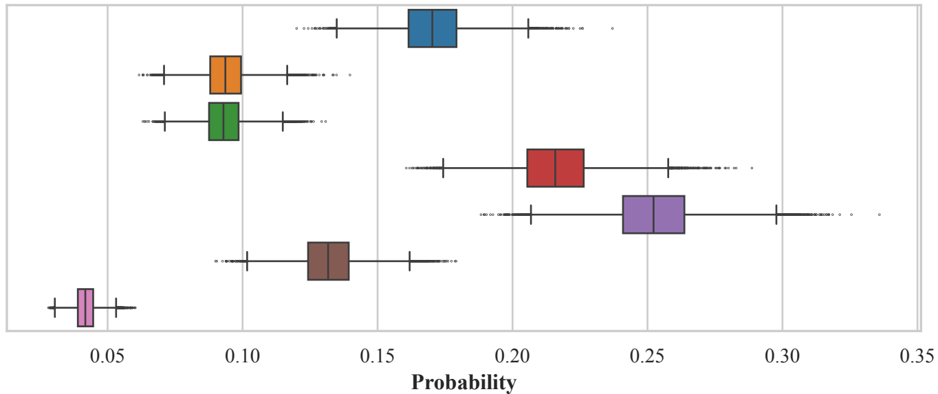
Model Complexity
