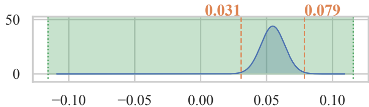
Concrete Strength
