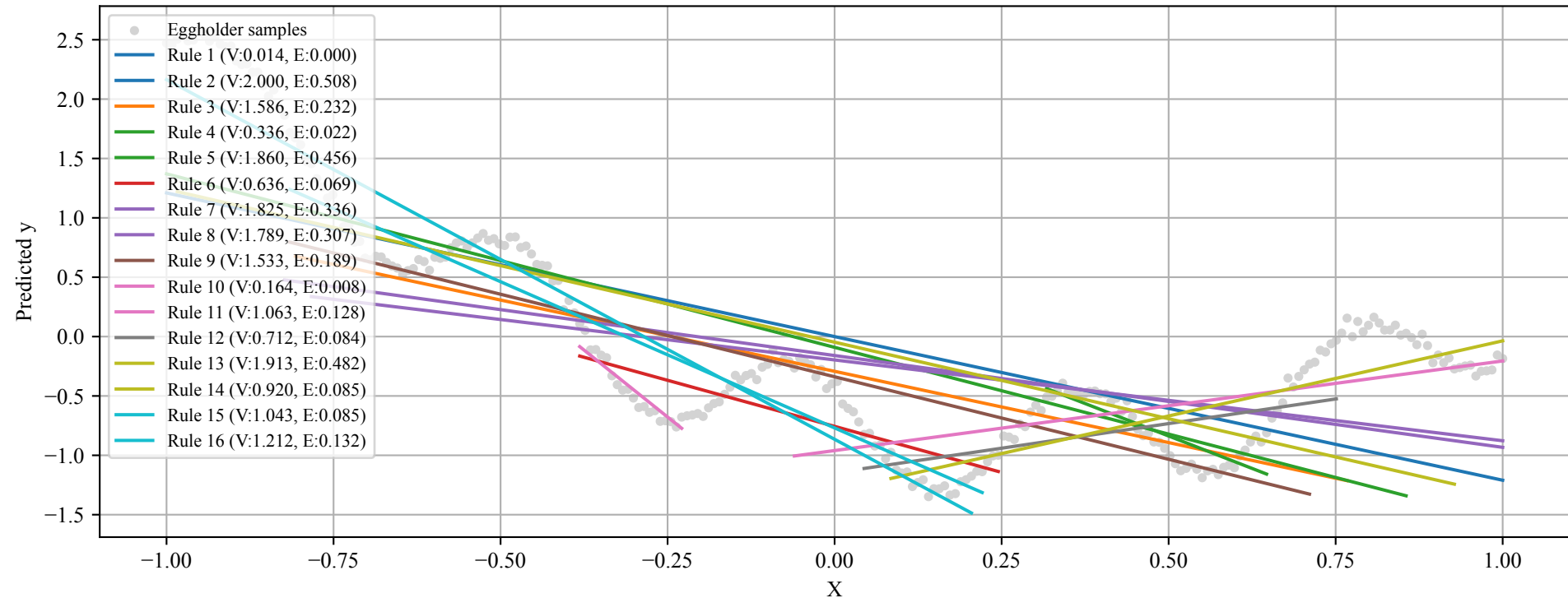
Rule Predictions on Eggholder Samples - NSGA2+Volume
