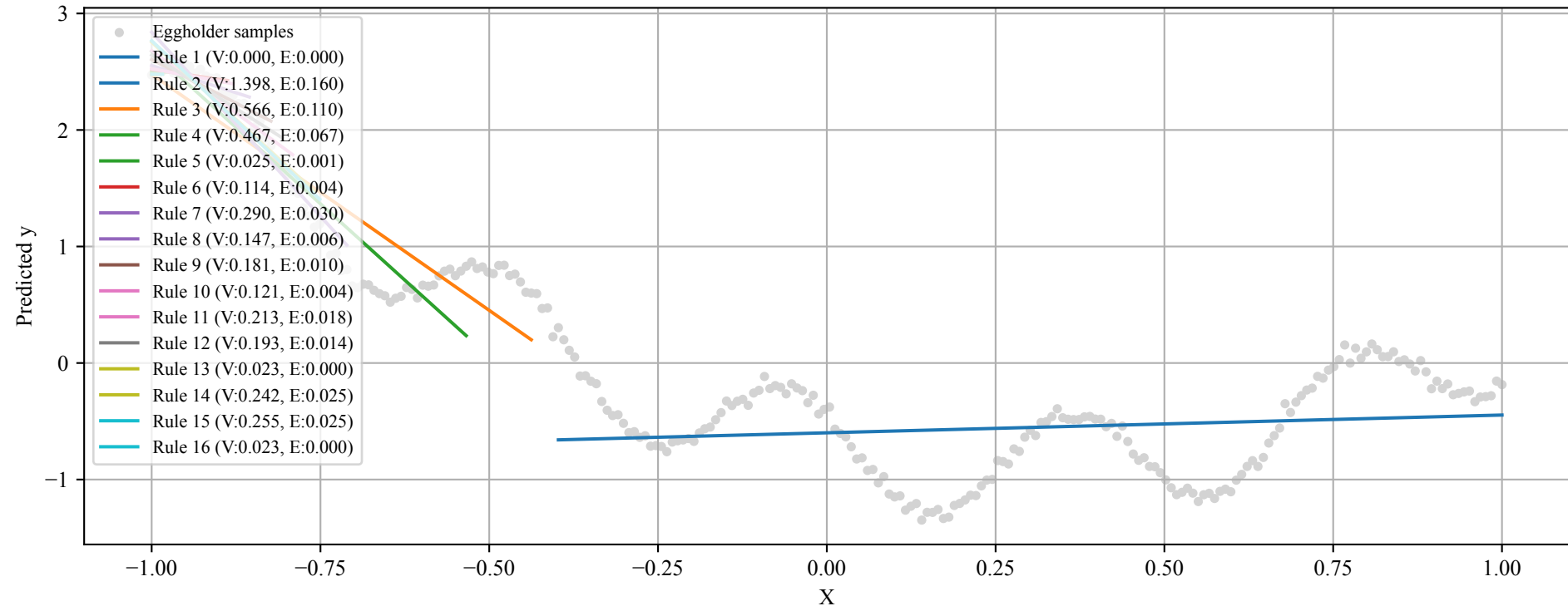
Rule Predictions on Eggholder Samples - NSGA2+Variance Reduction
