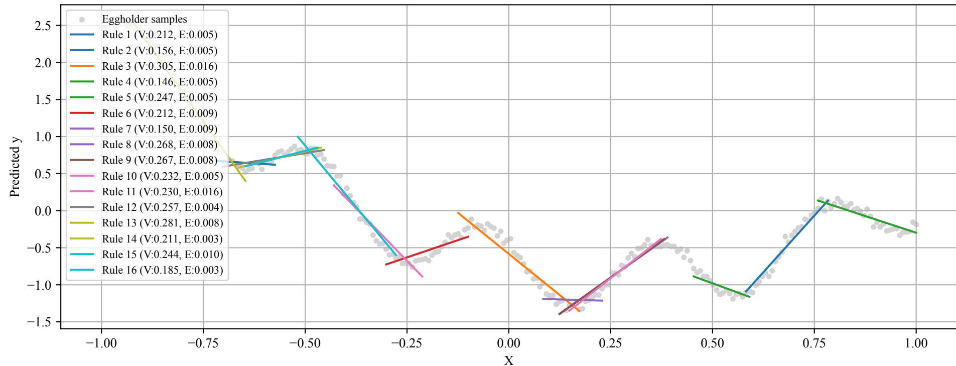
Rule Predictions on Eggholder Samples - ES Baseline
