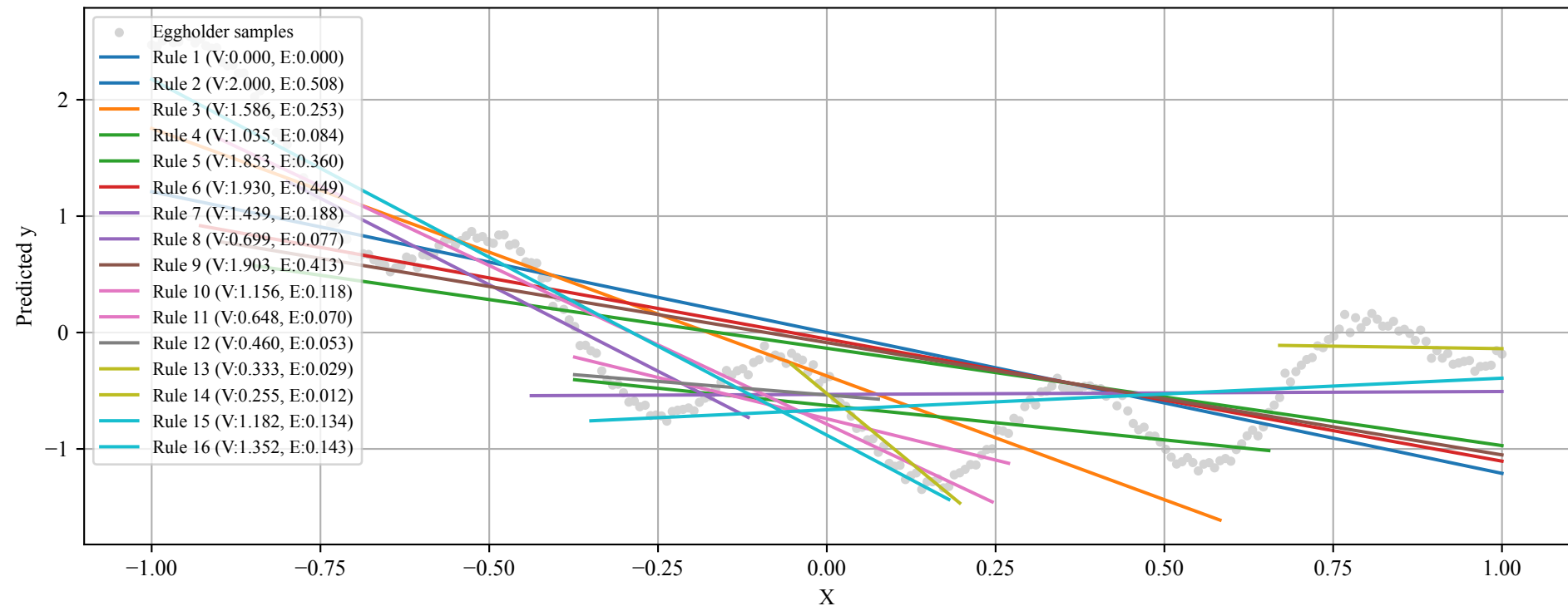
Rule Predictions on Eggholder Samples - NSGA2+Support
