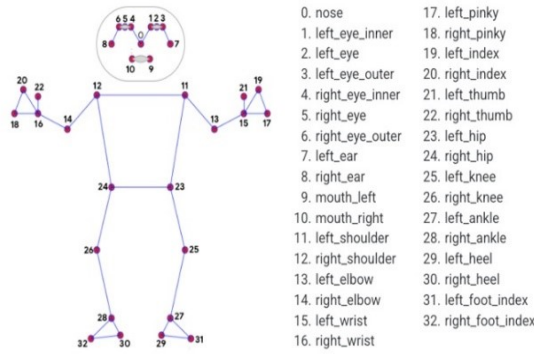
Fig. 1. BlazePose 33 Keypoints topology [18]
