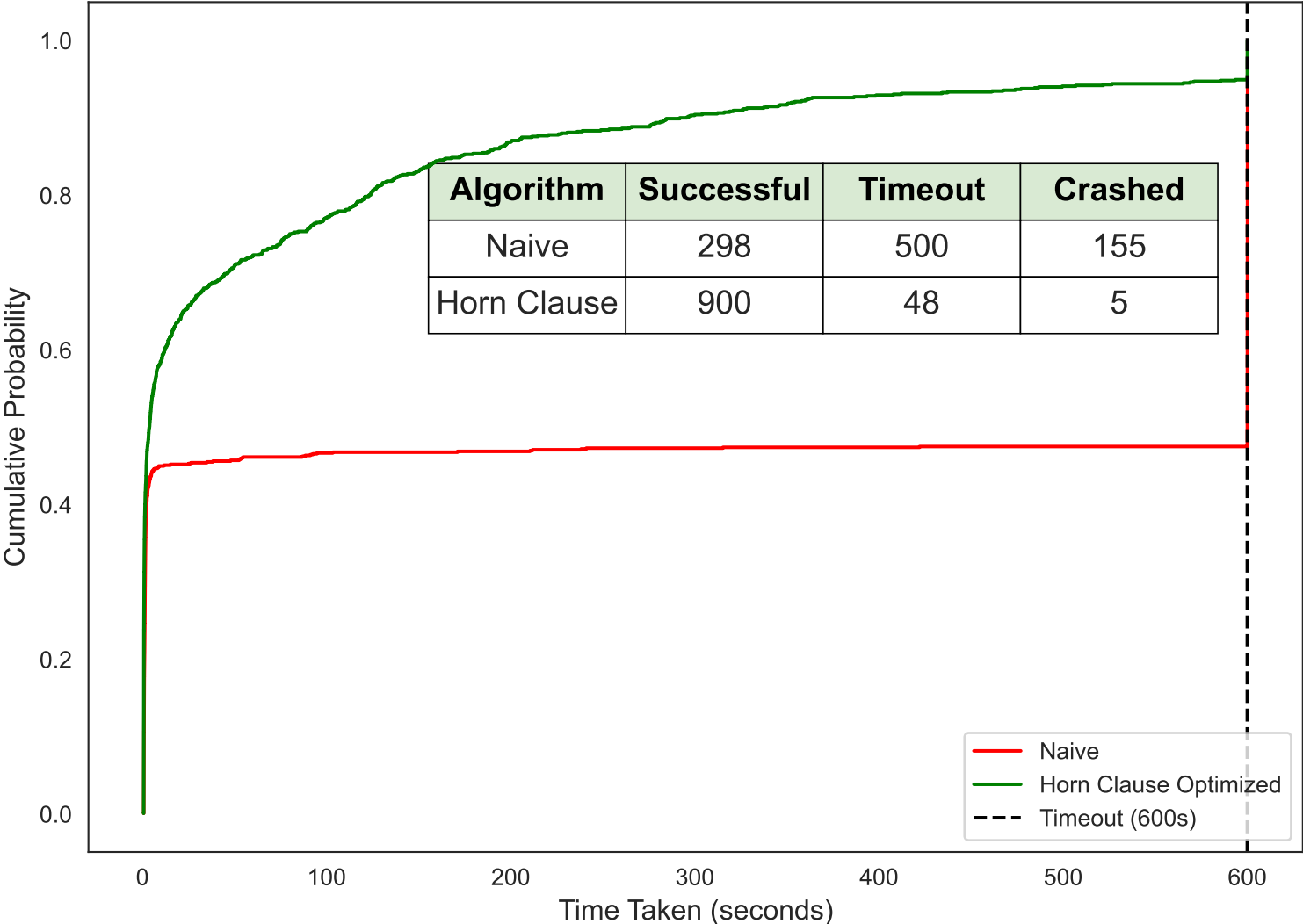
CDF of Execution Time (with Timeouts)
