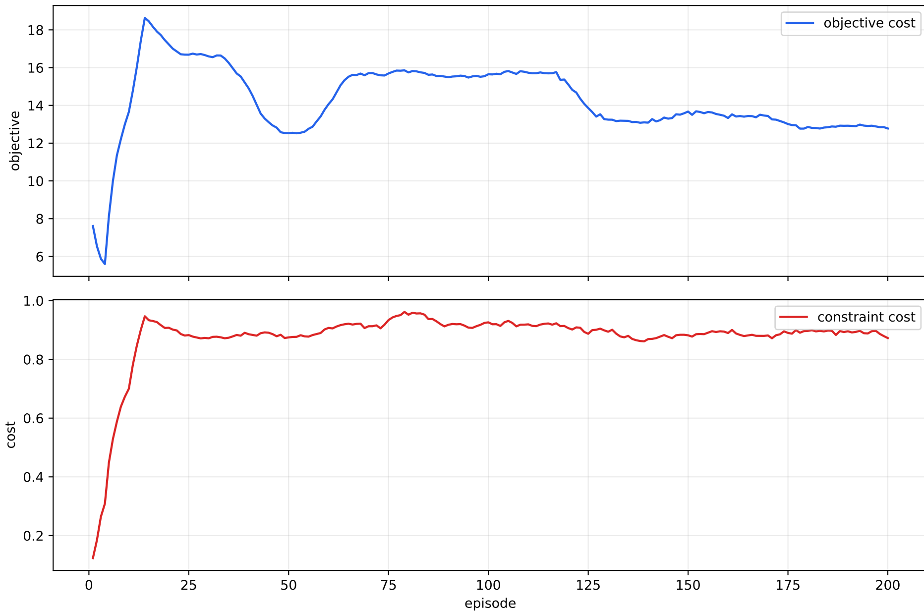
MultiCell CTDE dB-action SLDAC 200 episodes
