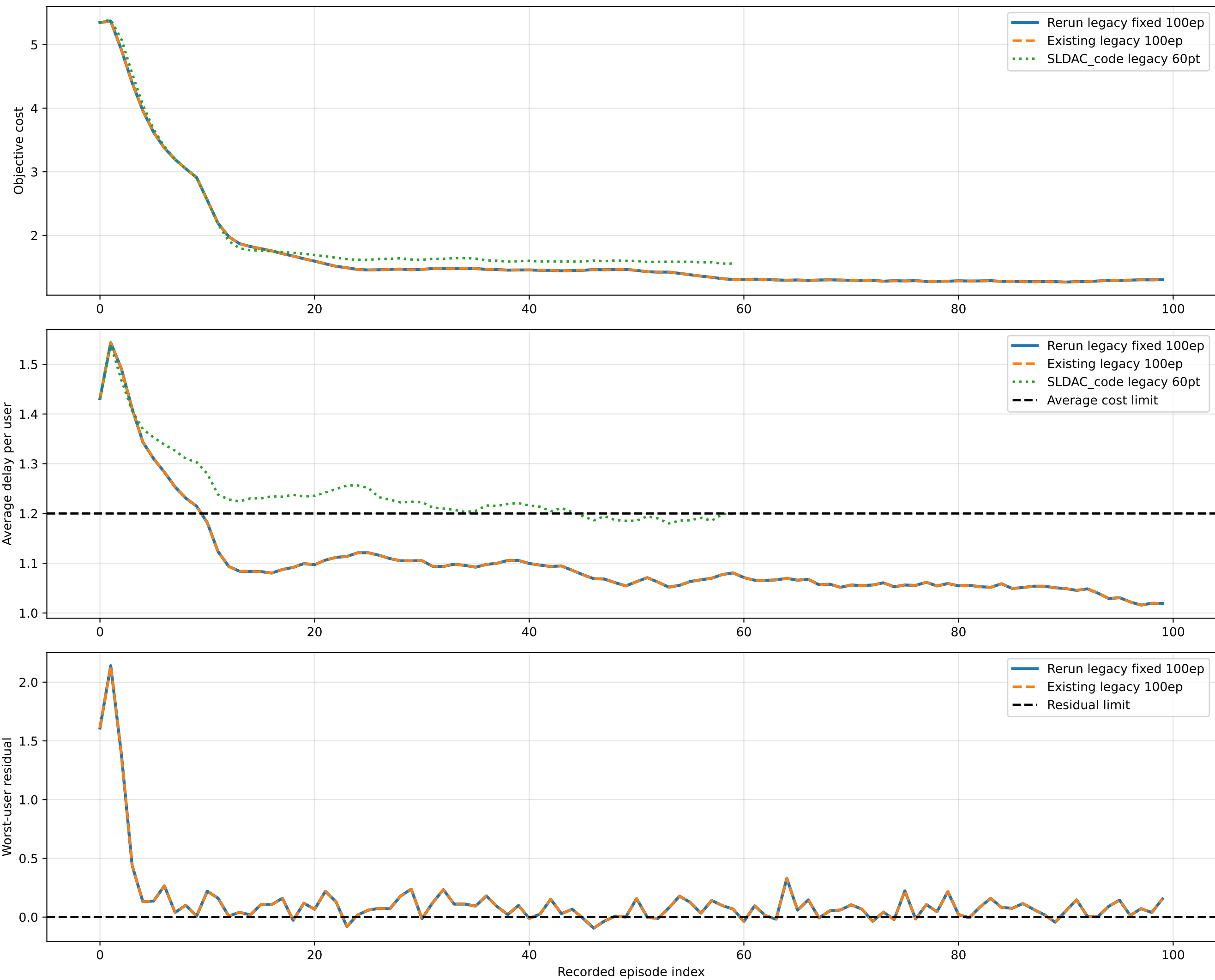
Legacy SLDAC fixed MIMO critic rerun b100_q1 100ep
