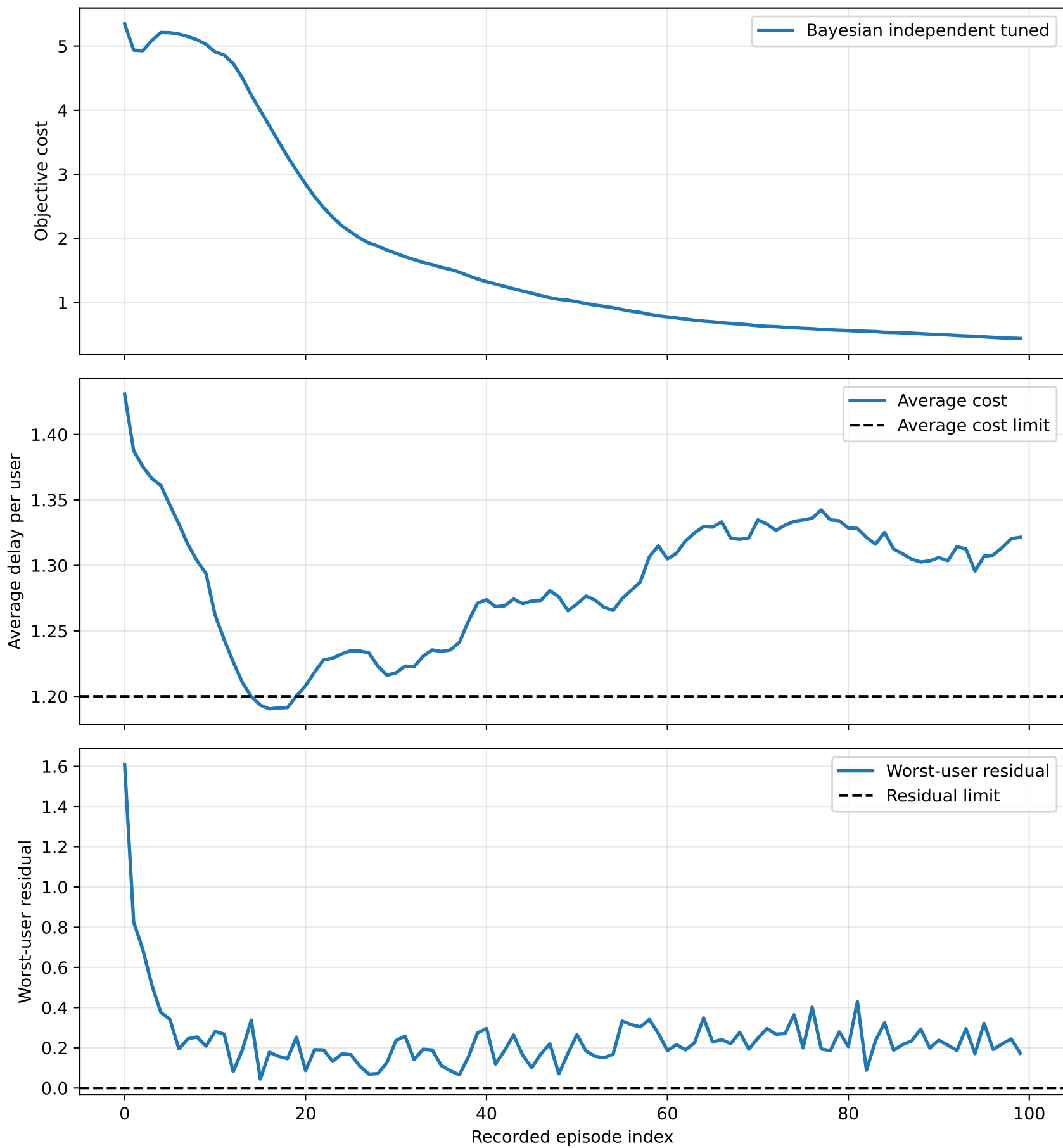
Independent Bayesian SLDAC b100_q1 100ep
