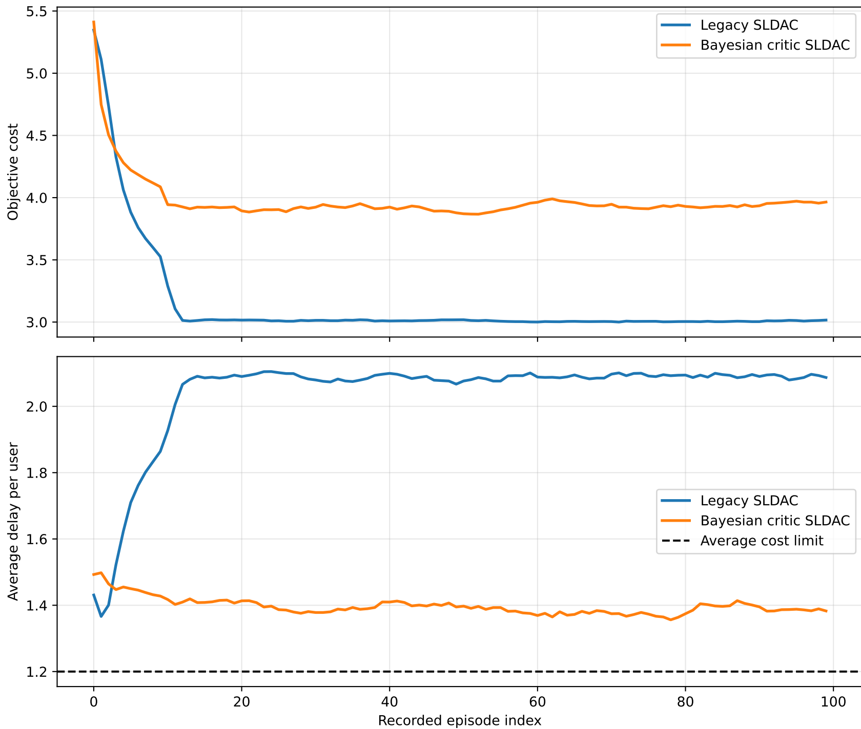
b100_q1 100-episode comparison
