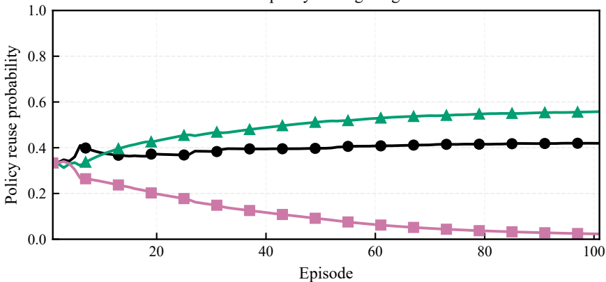
HRL policy mixing weights
