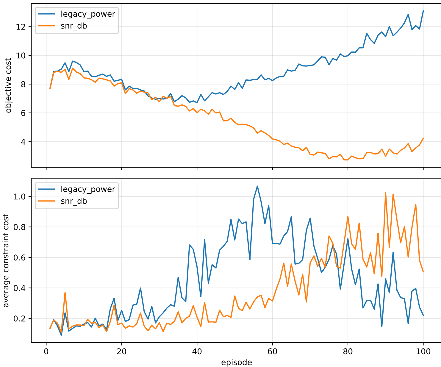
Tree CTDE-SLDAC 100ep: legacy_power vs snr_db
