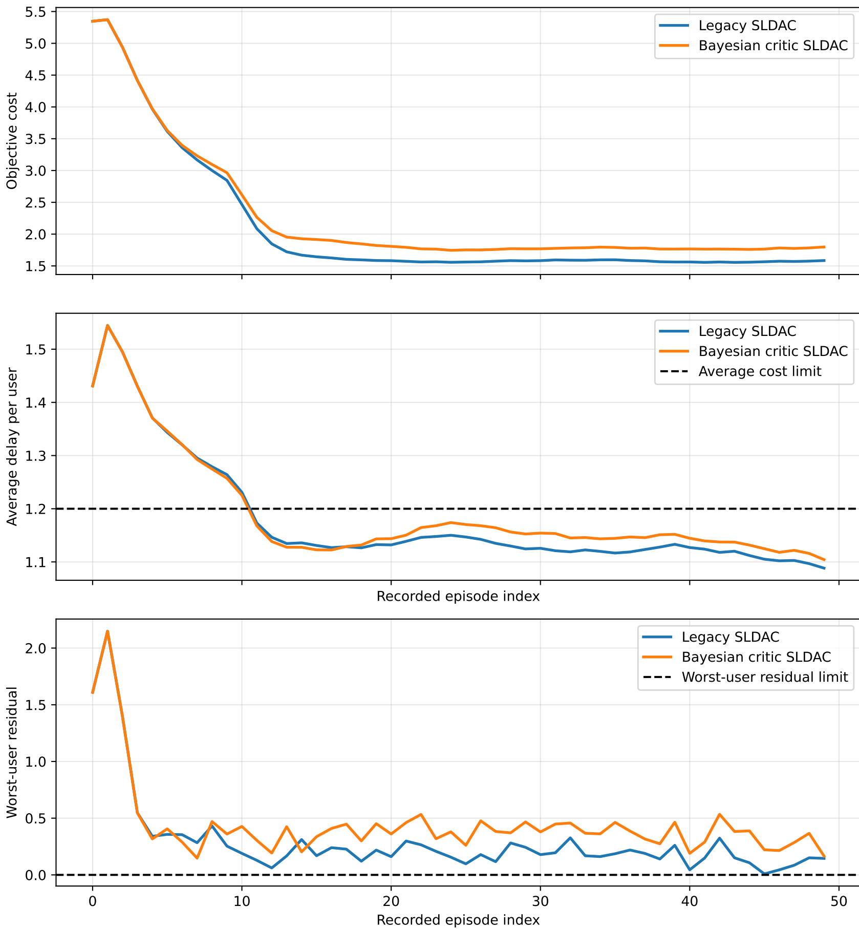
b100_q1 50-episode comparison
