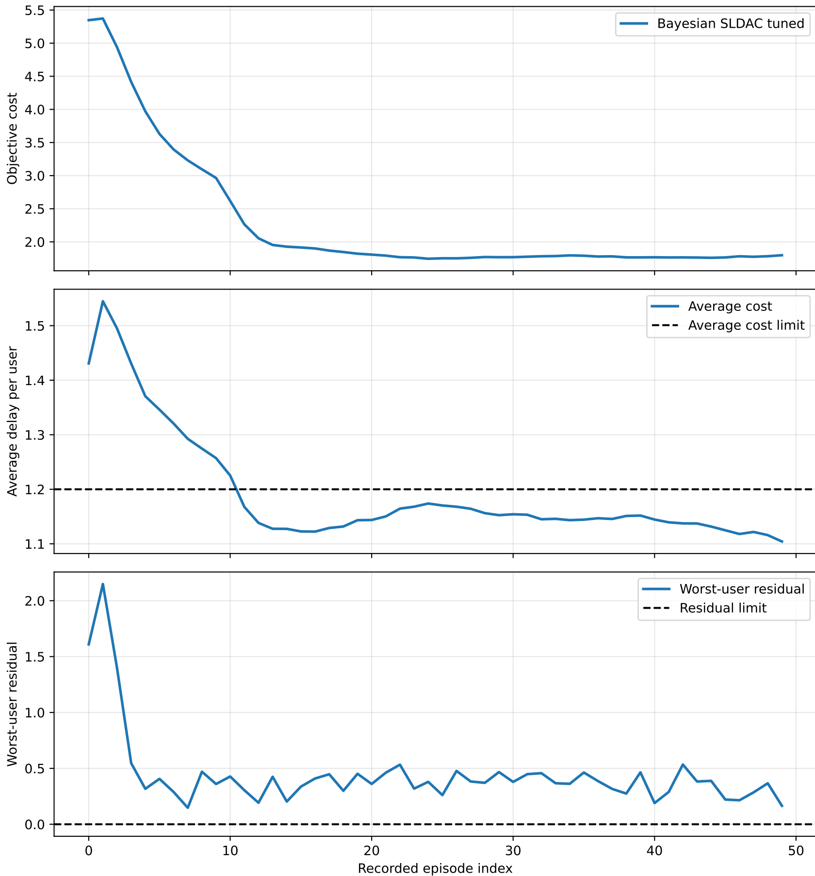
Bayesian SLDAC b100_q1 50ep
