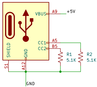
J1 USB_C_Receptacle_PowerOnly_6P
