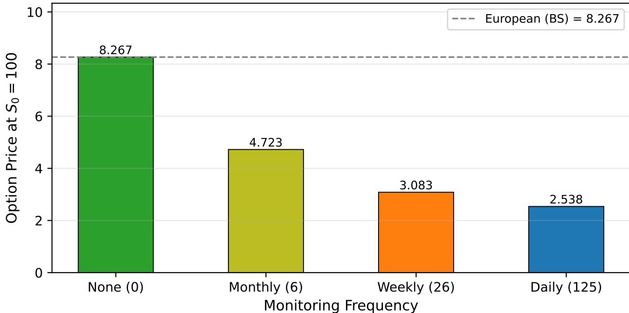
Barrier Price vs Monitoring Frequency ( K = 100 , T = 0.5 , r = 0.1 , \sigma = 0.2 , S_L = 95 , S_U = 125 )
