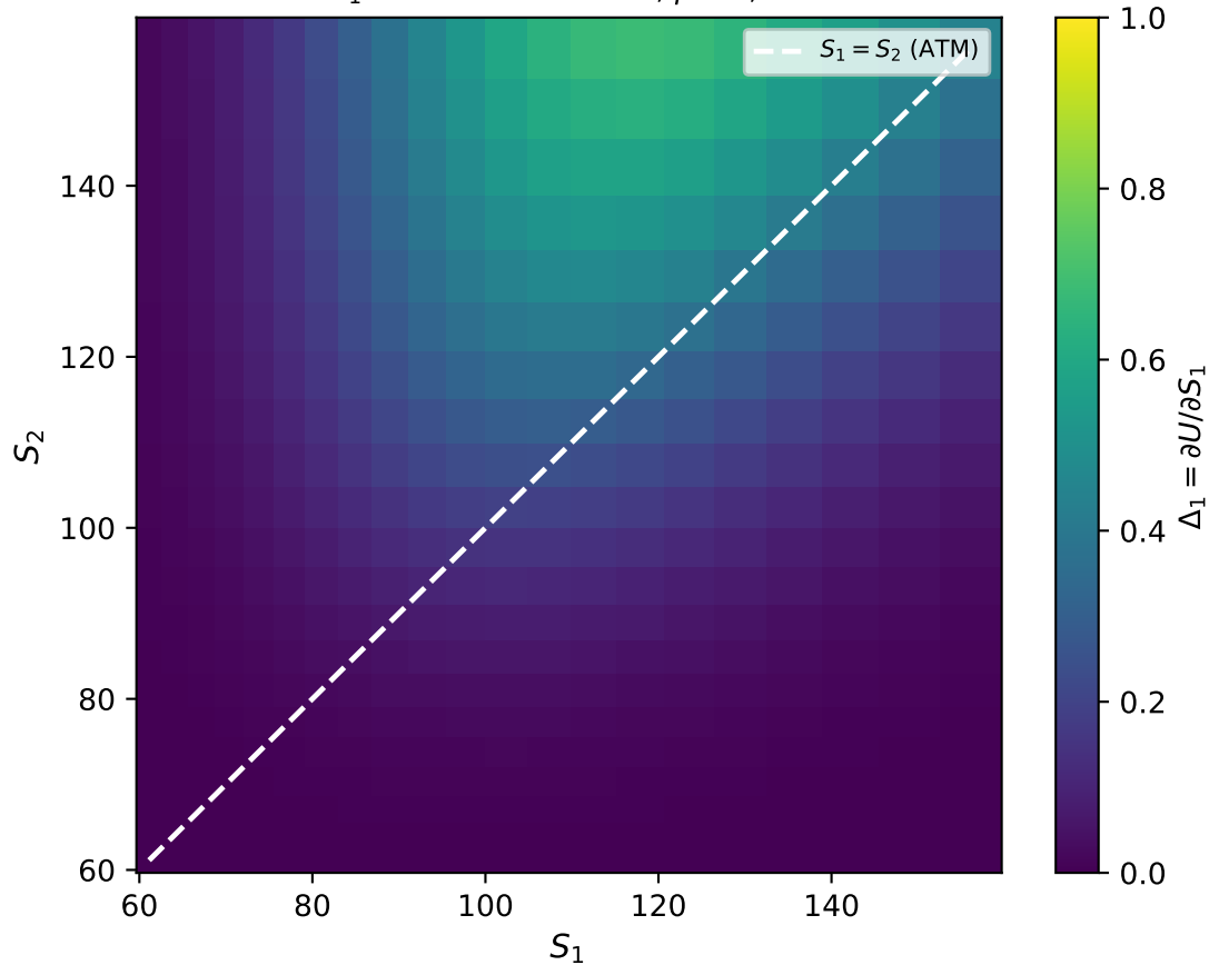
DPG \Delta_1 : call-on-min basket, \rho = 0 , N = 256
