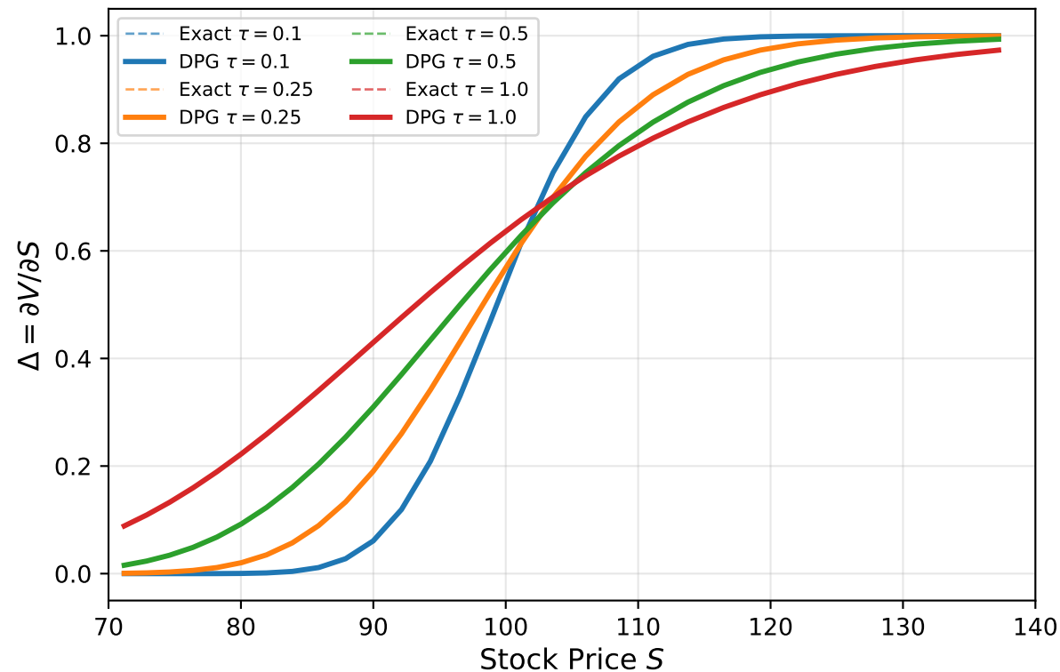
European Call Delta (V2 Ultraweak DPG, \sigma = 0.20 )
