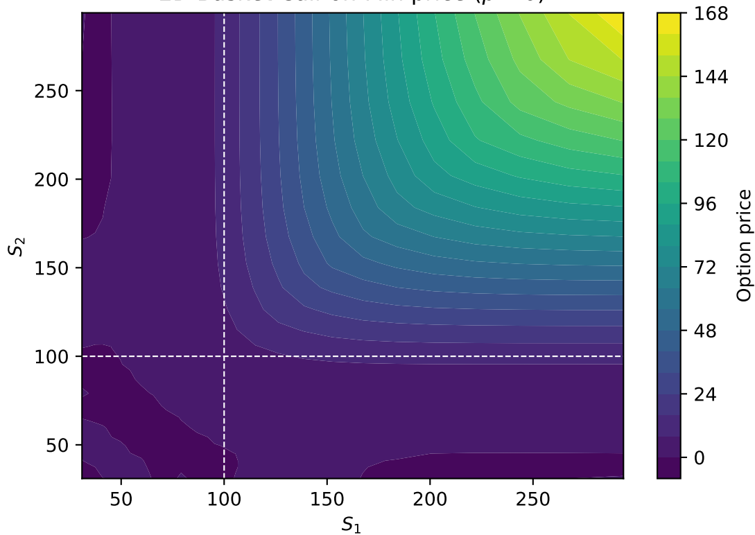
2D Basket Call-on-Min price ( \rho = 0 )
