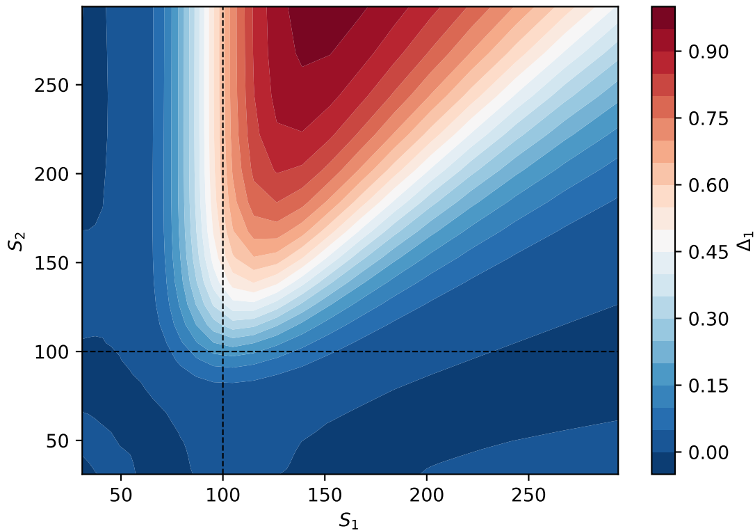
Delta 1 surface ( \rho = 0 )
