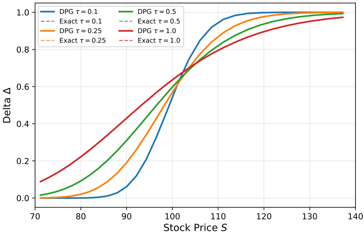
European Call Delta (V2 Ultraweak DPG, \sigma = 0.20 )
