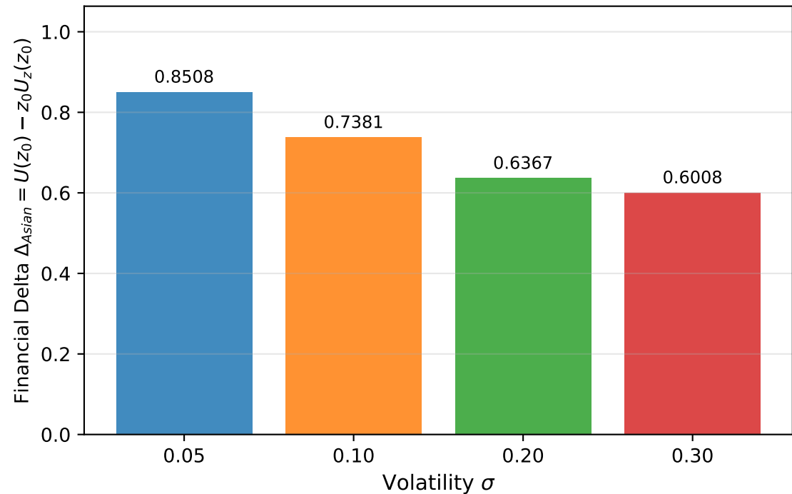
Asian Call Financial \Delta at z_0 = K/S_0 = 1.0
