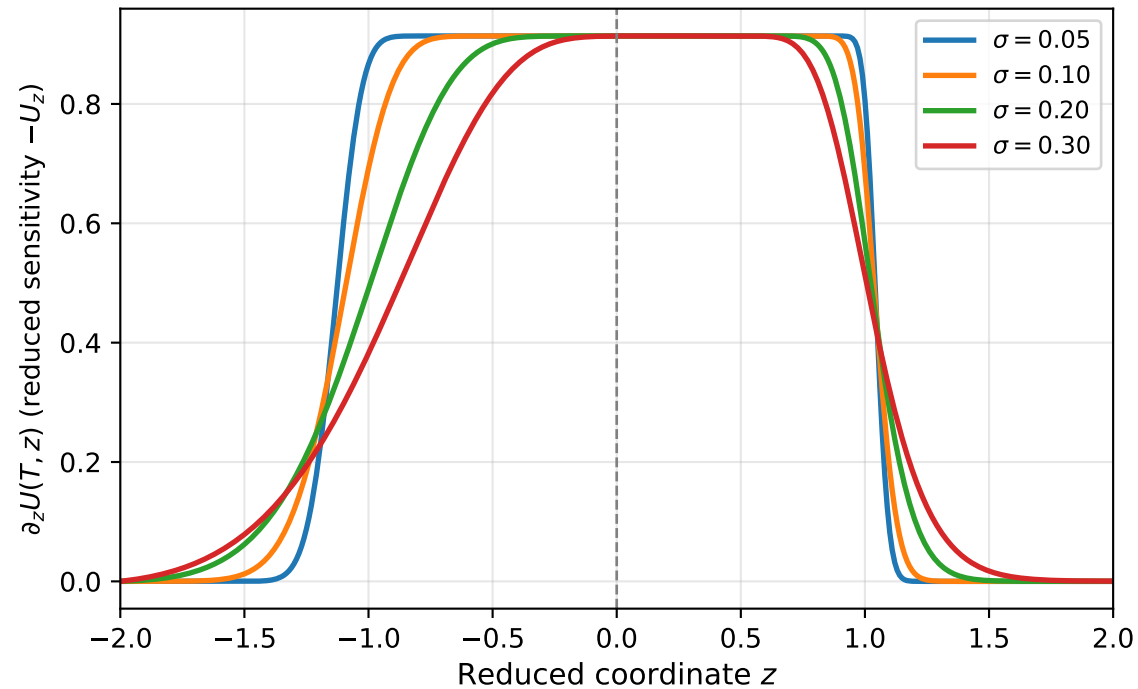
Reduced-Coordinate Sensitivity -U_z(T, z)
