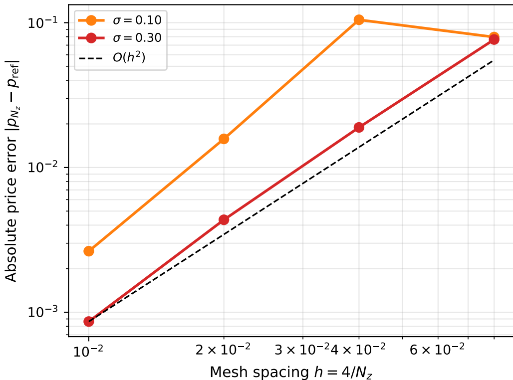
Asian Option Spatial Convergence (DPG p = 1 , r = 0.09 , N_t = 2000 , K = S_0 = 100 )
