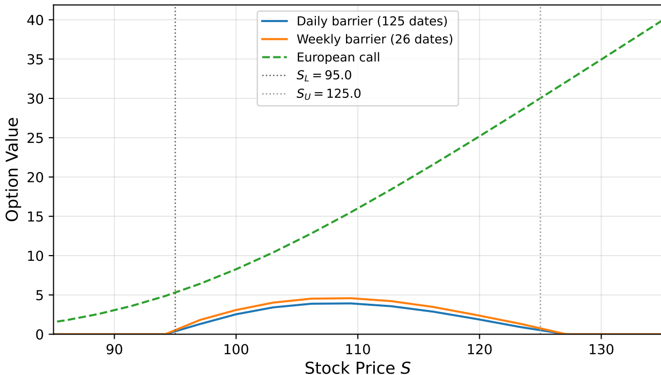
Discrete Double-Barrier Call Option Value ( K = 100 , T = 0.5 , r = 0.1 , \sigma = 0.2 , S_L = 95 , S_U = 125 )
