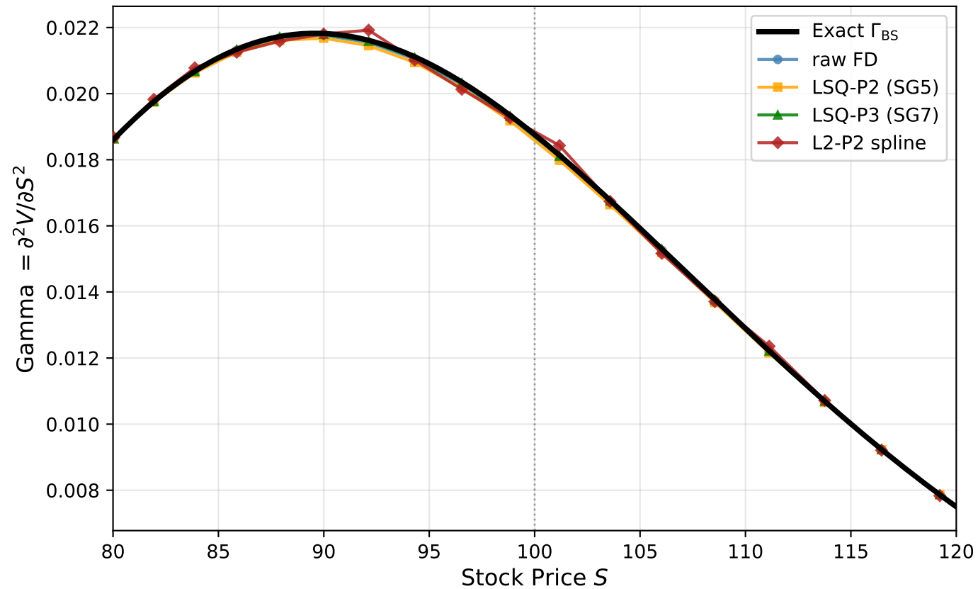
European call: Gamma recovery at N_x = 256
