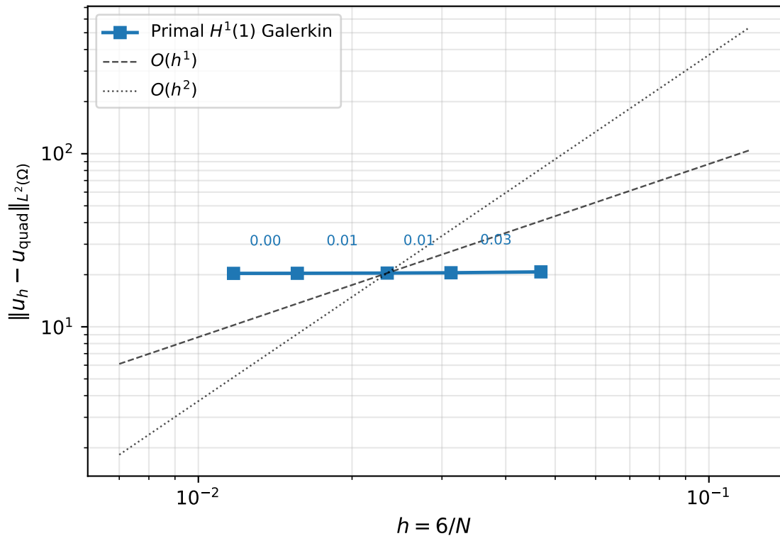
Basket-avg call: primal H^1(1) , \rho = 0.5 , N_t = 2N
