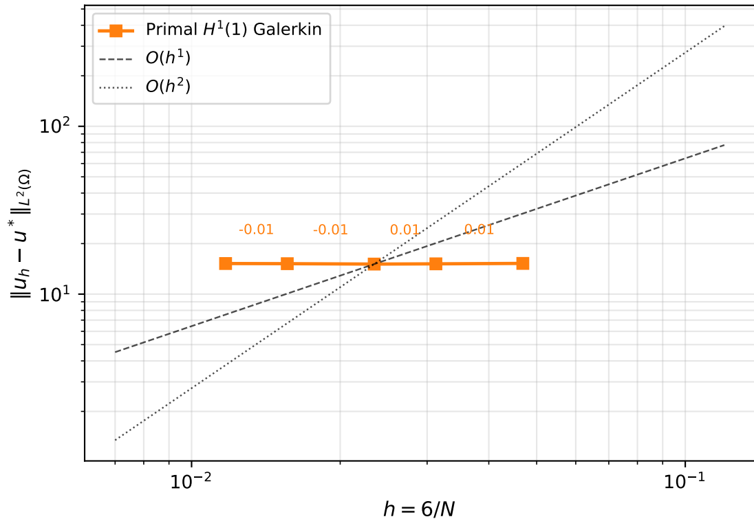
Best-of call (Stulz): primal H^1(1) Galerkin, \rho = 0.5 , N_t = 2N
