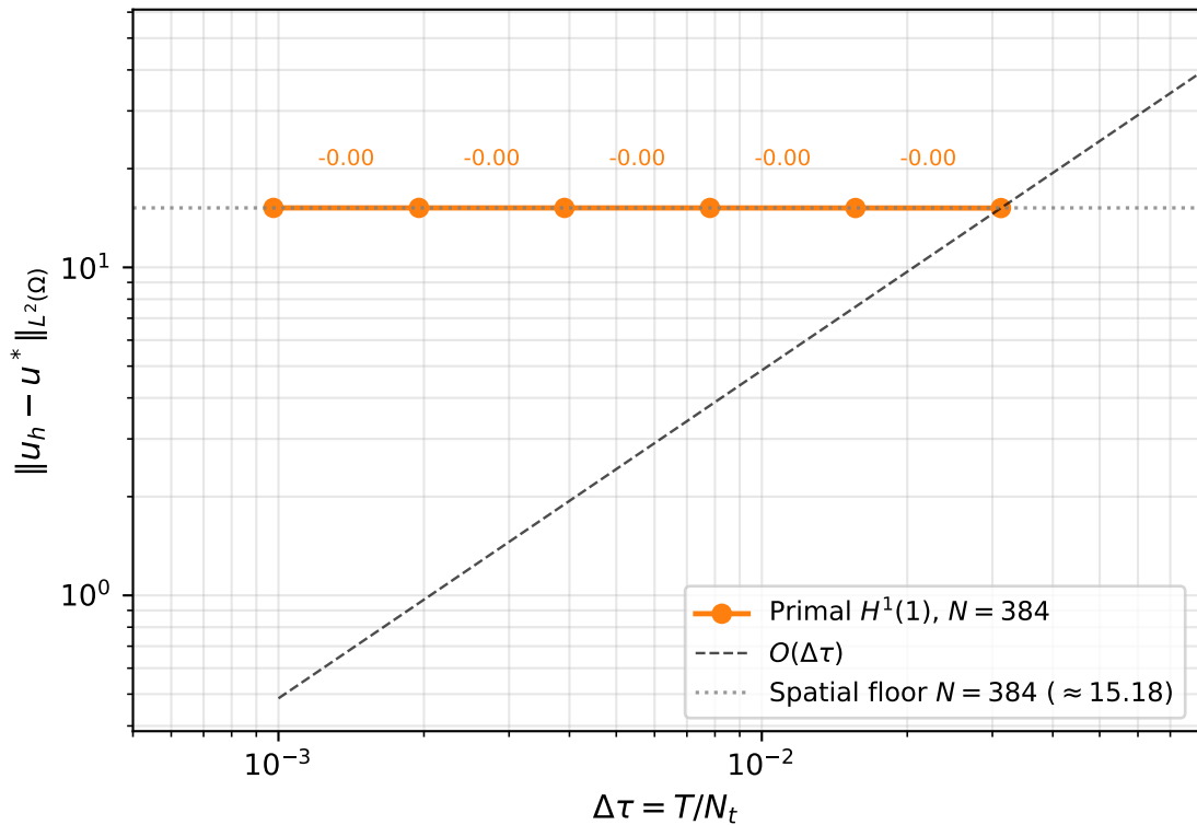
Best-of call: primal H^1(1) , temporal convergence, N = 384
