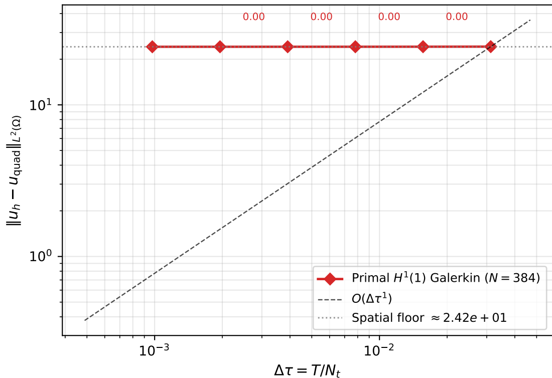
Spread call ( \tilde{K} = 10 ): primal H^1(1) , N = 384 , \rho = 0.5
