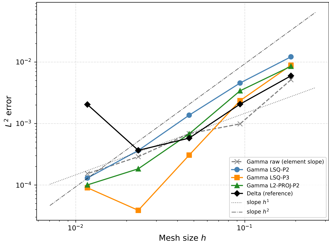
Gamma recovery — European call, \sigma = 0.20
