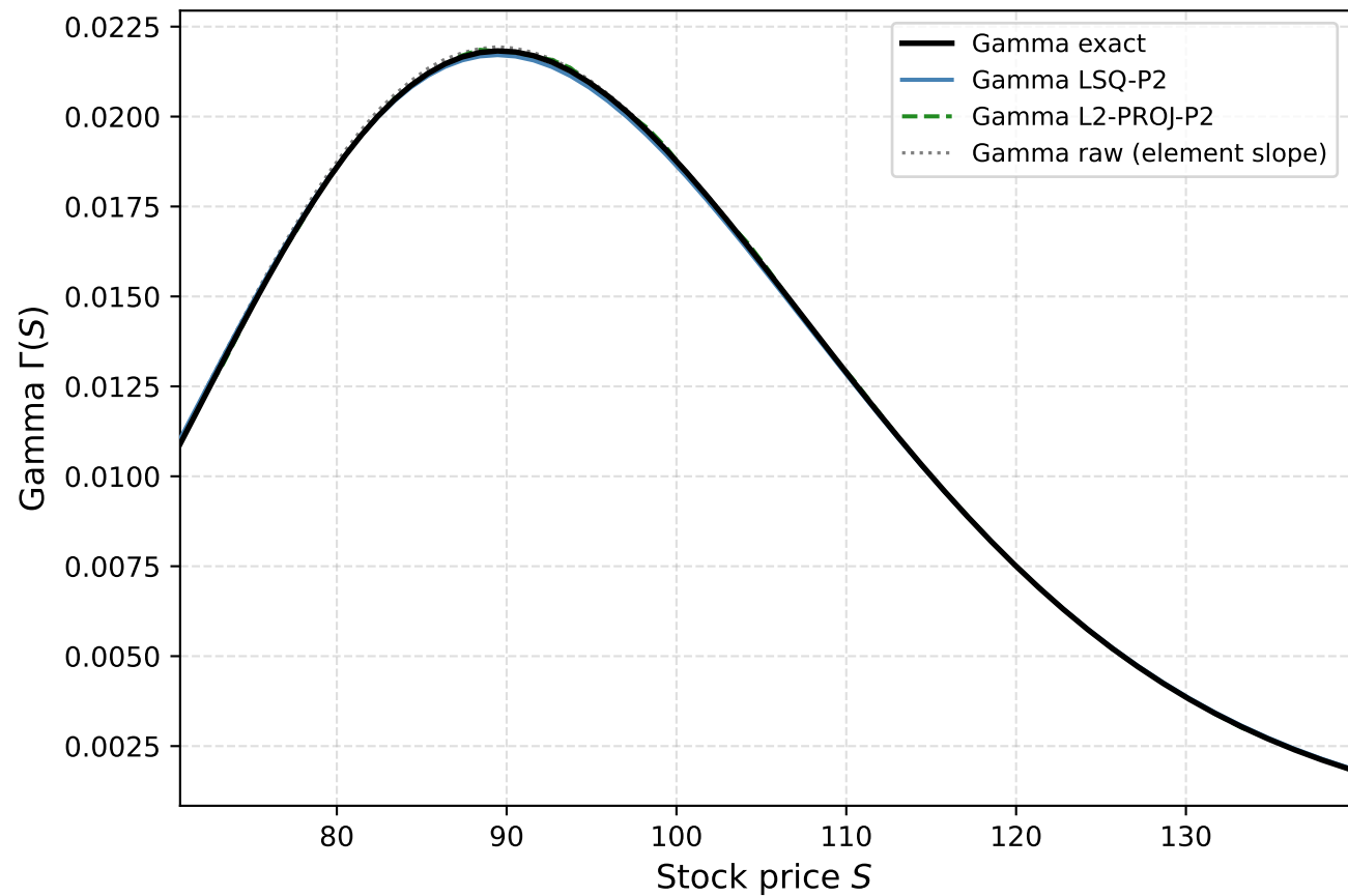
Gamma profiles at N_x = 512 — European call, \sigma = 0.20
