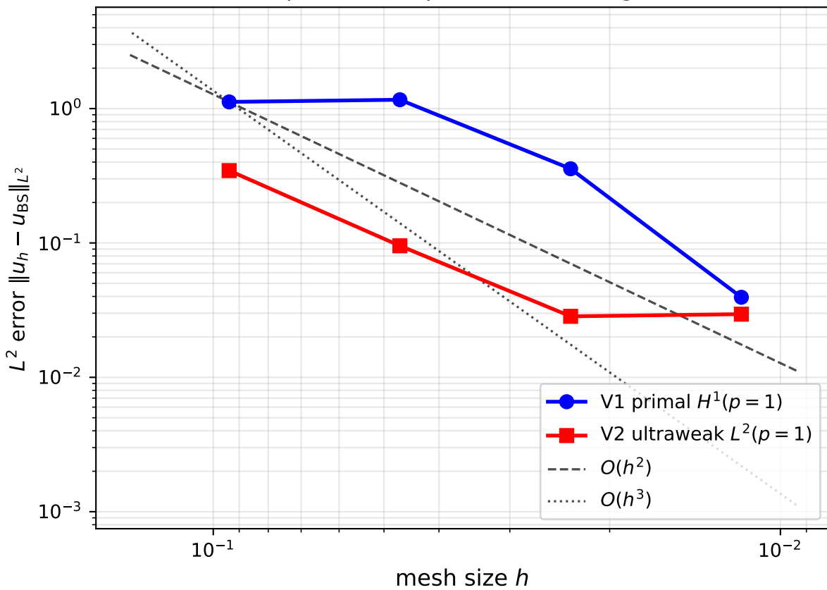
European call: spatial L^2 convergence
