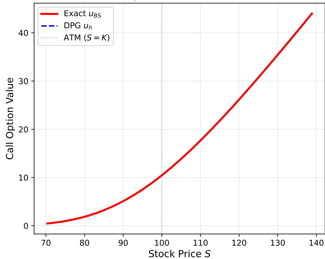
European call: DPG vs exact
