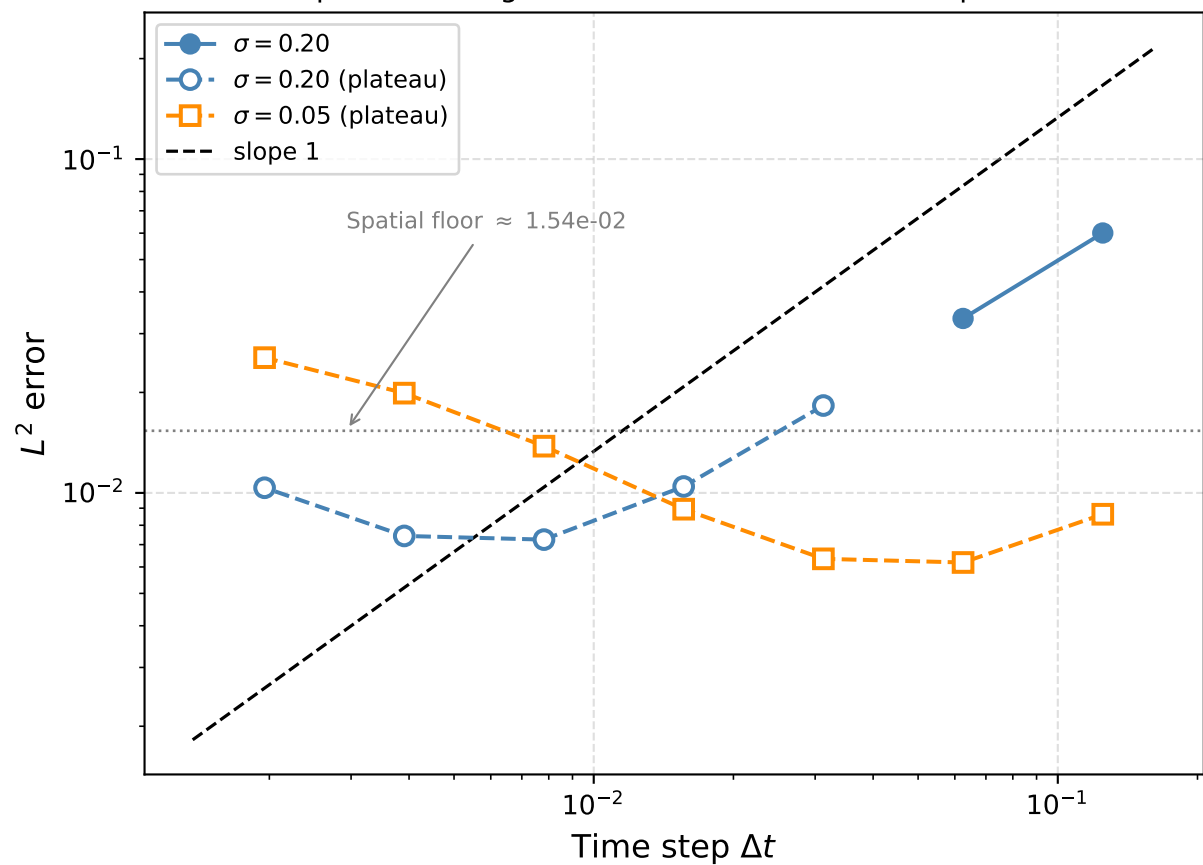
Temporal convergence: V2 ultraweak DPG, European call
