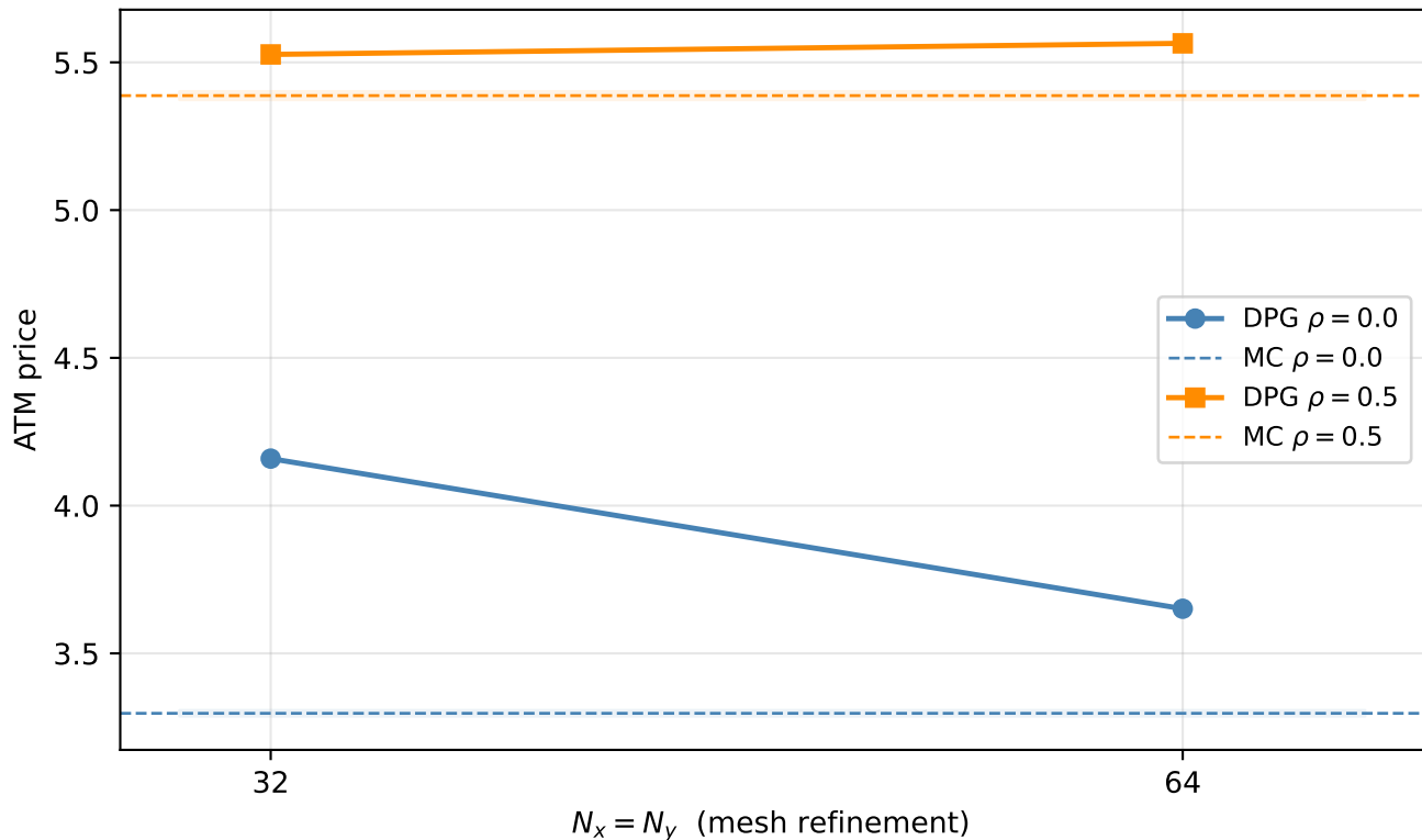
2D Basket Call-on-Min: DPG convergence to MC (K=100)
