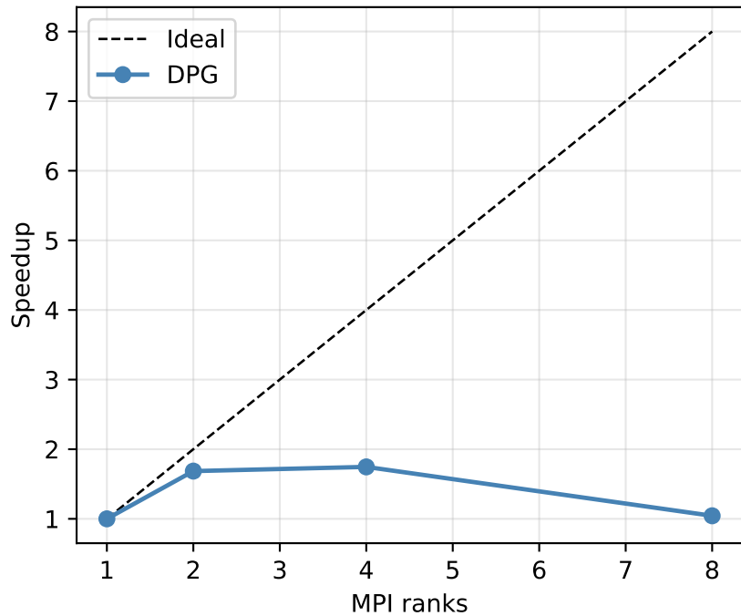
Strong-scaling speedup
