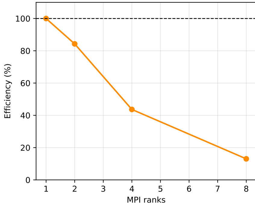
Parallel efficiency
