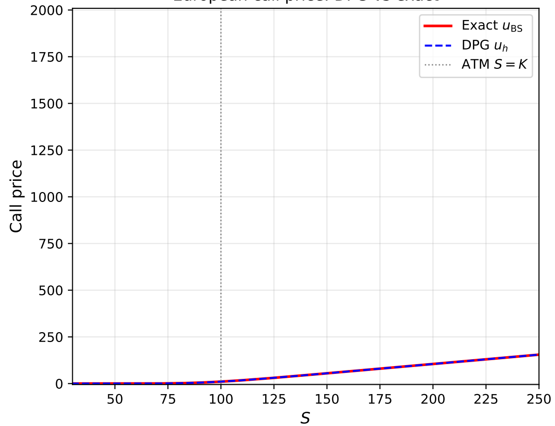
European call price: DPG vs exact
