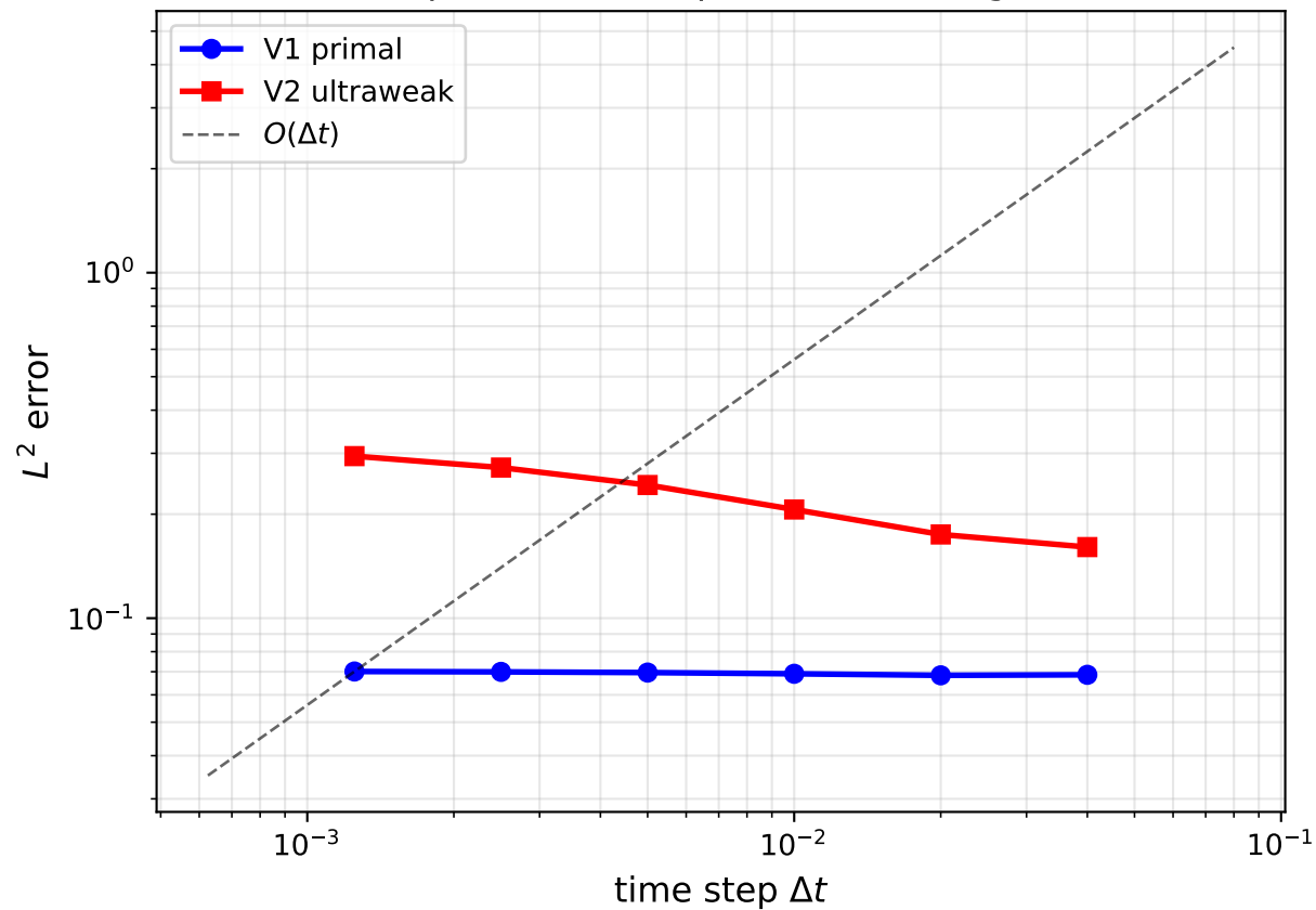
European call: temporal L^2 convergence
